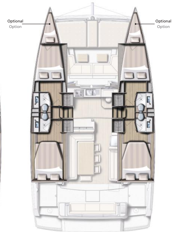
4 CABINS / 4 HEADS VERSION
